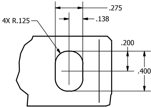
DETAIL B SLOT 2 PLACES
